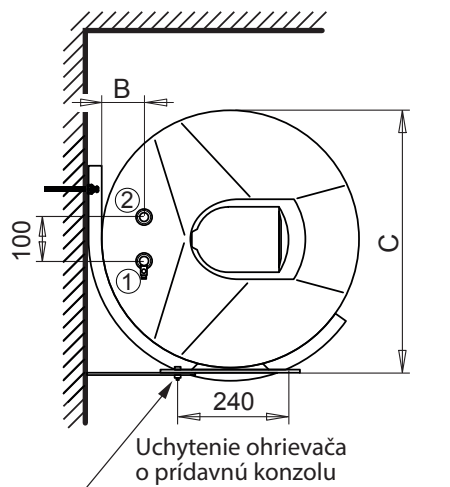
Obr. 5 - model EURO 150 X, 200 X
