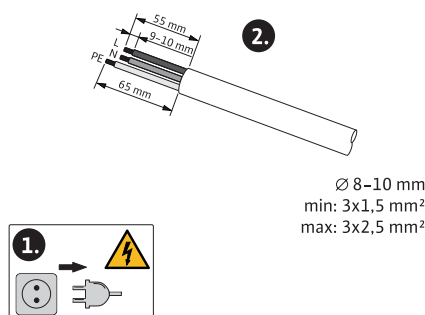
Fig. 21: Preparing the connection
