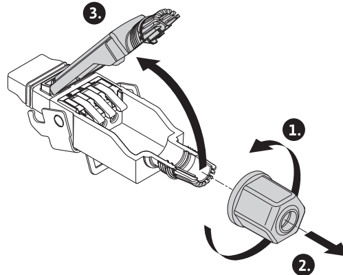
Fig. 25: Open Wilo-Connector
