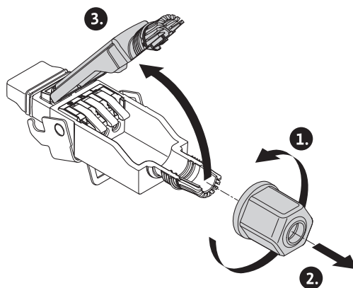
Fig. 25: Otvaranje Wilo-Connector-a
